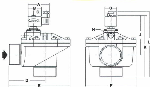
Fig. 3: External threaded type - aluminium
